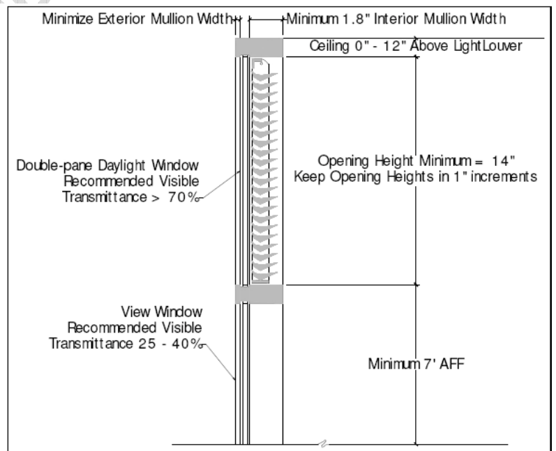
Figure 2: Schematic Section of LightLouver Unit Installation
